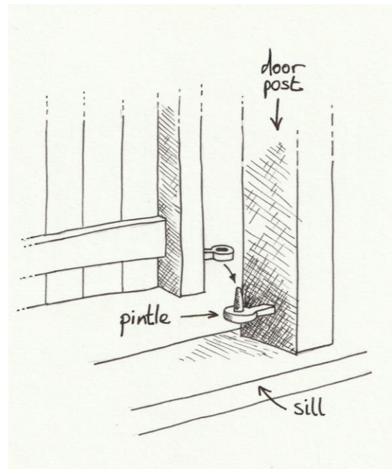
(left) The protruding 'harr' on the door slots into sockets in a timber or stone sill and lintel. (right) A metal pintle is set into a stone or timber post, and the door hinge pivots on it – there are several types of design. (© PDNPA)
