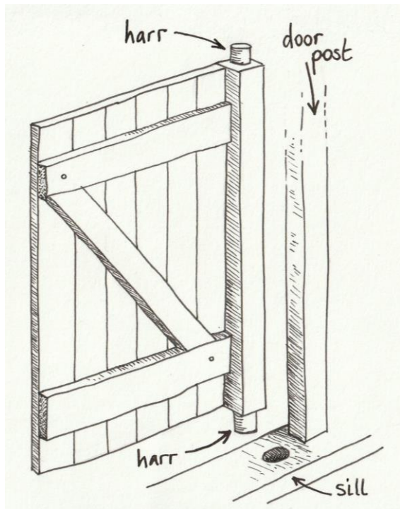
(left) The protruding 'harr' on the door slots into sockets in a timber or stone sill and lintel. (right) A metal pintle is set into a stone or timber post, and the door hinge pivots on it – there are several types of design. (© PDNPA)
